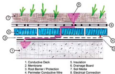
Figure 4 - ELD section with overburden in place.
