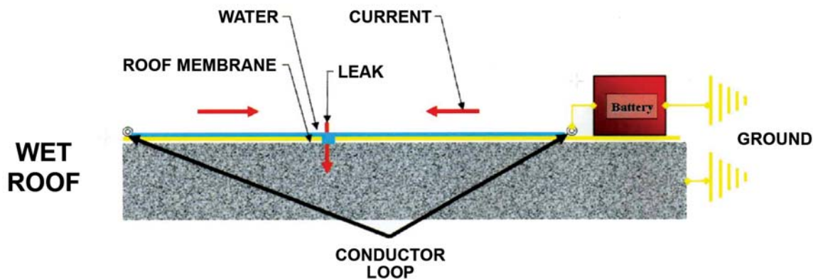
Figure 1 – The surface of the waterproofing must be wetted to provide an electrically conductive medium.
